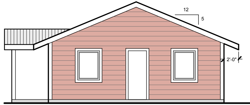
RIGHT ELEVATION 1/8" = 1'-0"
