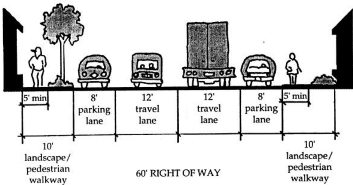
FIGURE 3.6 LOCAL ROADS STREETSCAPE CROSS-SECTION
